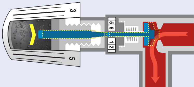
05 Thermostatventil
