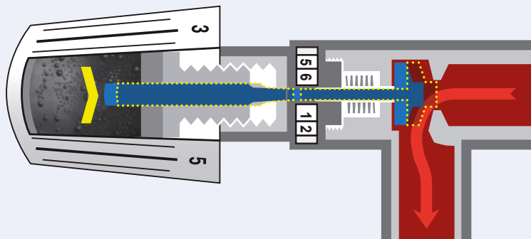
05 Thermostatventil
